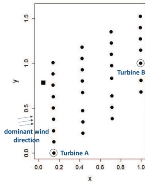
Figure 1. Wind farm layout.
