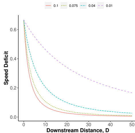
Fig 2: Influence of wake decay parameter on wind speed deficit in Jensen's wake model in a two-turbine setting. The downstream distance on the x -axis refers to the distance between upstream and downstream turbines.
