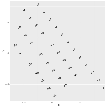
Fig 6: Layout of WF 1. Solid circles represent turbine locations.
